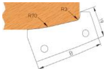
Art.-Nr./item no./num. art. 09.1442 Abmessung/dimensions/dimensions 40 x 20 x 2 mm
