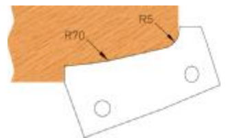
Art.-Nr./item no./num. art. 09.1445 Abmessung/dimensions/dimensions 40 x 20 x 2 mm
