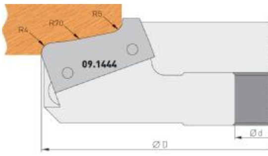
Art.-Nr./item no./num. art. 09.1444 Abmessung/dimensions/dimensions 40 x 20 x 2 mm
