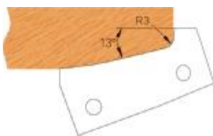
Art.-Nr./item no./num. art. 09.1441 Abmessung/dimensions/dimensions 40 x 20 x 2 mm
