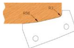
Art.-Nr./item no./num. art. 09.1443 Abmessung/dimensions/dimensions 40 x 20 x 2 mm
